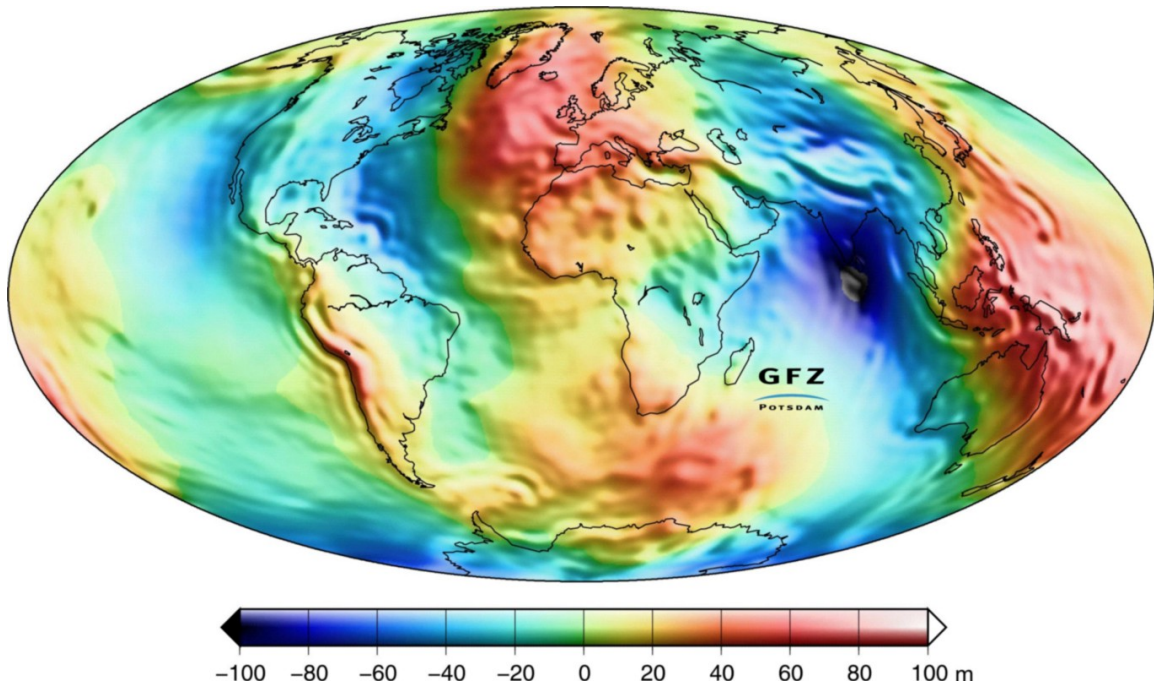
Image credit: NASA / GRACE mission / Christoph Reigber, et al. (2005): An Earth gravity field model complete to degree and order 150 from GRACE: EIGEN-GRACE02S, Journal of Geodynamics 39(1),1–10. Reds indicate greater gravitational anomalies; blues are smaller ones.
